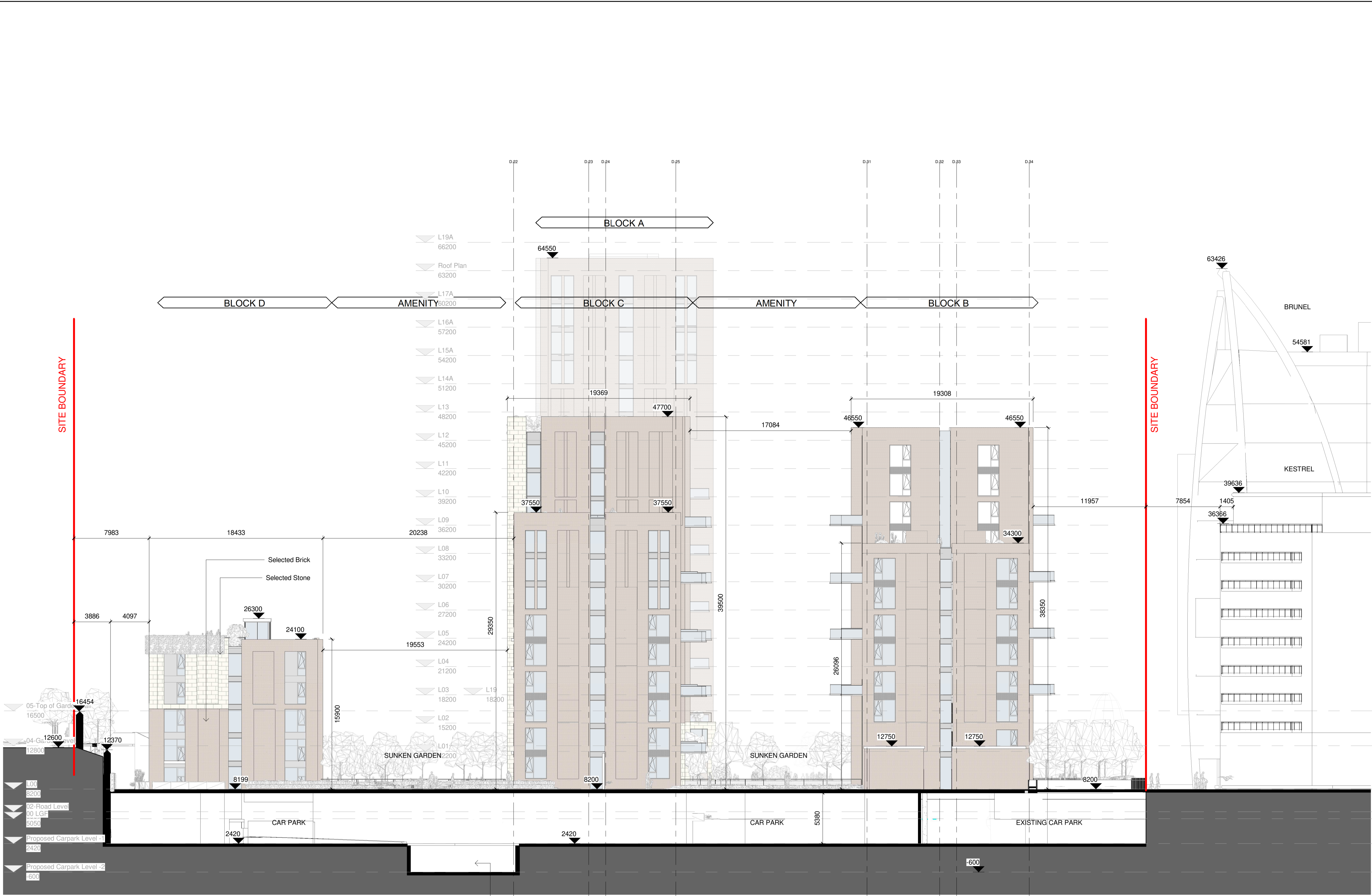
Proposed Elevation II 1:200
